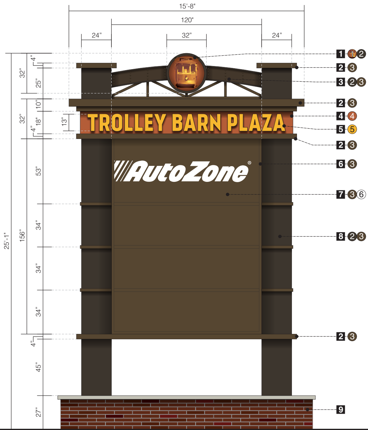
A Pylon Sign - Face View Scale: 1/4" = 1'-0"
